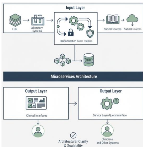
Fig 3: A Modular, Standards-Based Architecture for Clinical Decision Support Systems: Leveraging Microservices and FHIR for Interoperable Input-Output Pipelines
